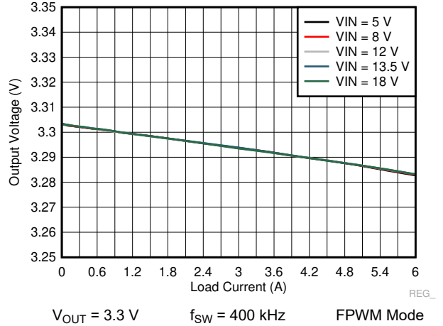
图 9-28. LM73606-Q1 Load and Line Regulation
