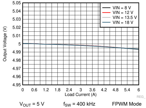
图 9-22. LM73606-Q1 Load and Line Regulation
