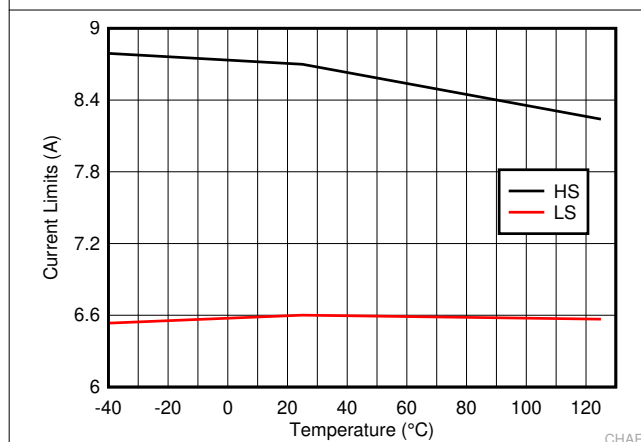
图 7-5. LM73605-Q1 High-Side and Low-Side Current Limit
