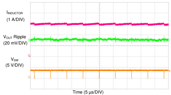
图 9-48. LM73606-Q1 Switching Waveform and V_{OUT} Ripple
