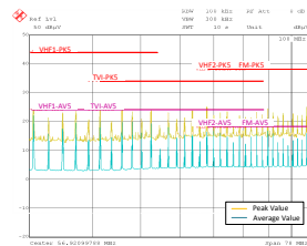
图 9-64. LM73606-Q1 Conducted EMI Result versus CISPR25 Limits - High Frequency
