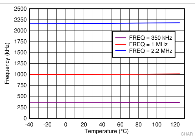
图 7-6. Switching Frequency Set by R_T Resistor
