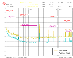
图 9-63. LM73606-Q1 Conducted EMI Result versus CISPR25 Limits - Low Frequency
