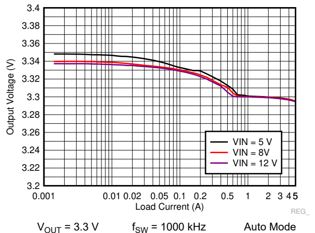
图 9-32. LM73605-Q1 Load and Line Regulation
