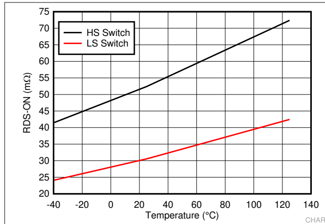
图 7-1. High-Side and Low-Side Switches R_{DS-ON}
