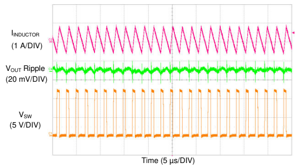
图 9-46. LM73606-Q1 Switching Waveform and V_{OUT} Ripple
