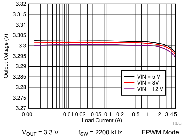
图 9-30. LM73605-Q1 Load and Line Regulation
