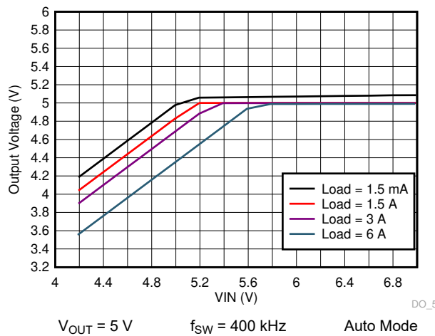
图 9-35. LM73606-Q1 Dropout Curve
