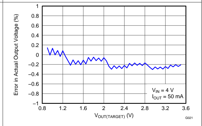
Figure 12. Accuracy vs Pin-Setting
