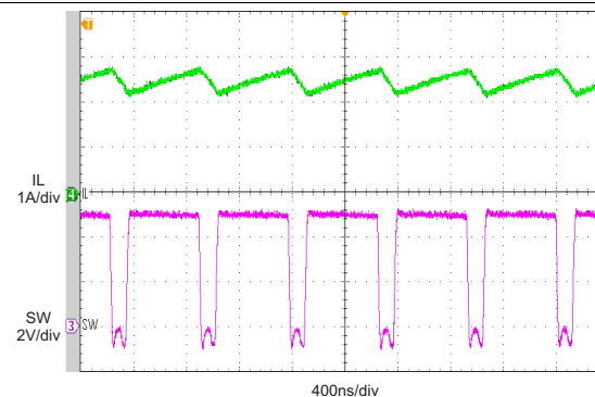
VBUS = 5 V, No Battery, ISYS = 40 mA, Charge Disable
