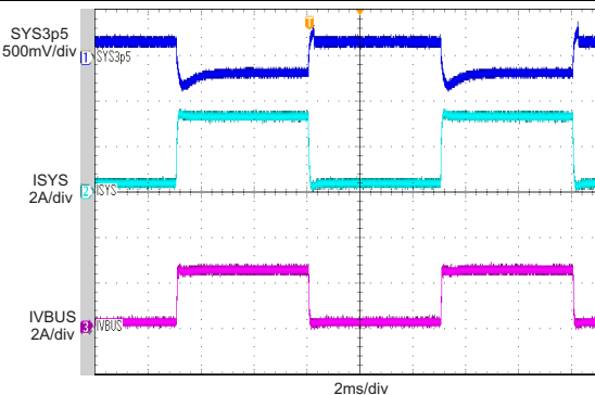
VBUS = 5 V, IIN = 3 A, No Battery, Charge Disable
