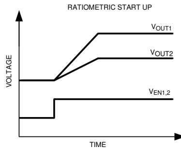
Figure 27. LM26420 Soft-Start
