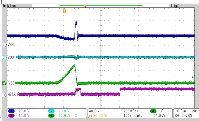
图 30. Device Version A Short Circuit Event
