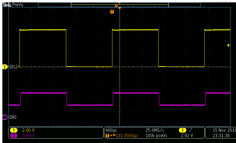
图 55. Toggling Between CH1 and CH2 Current Measurement
