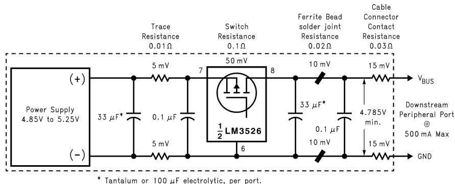
Figure 22. Self-Powered Hub Per-Port Voltage Drop
