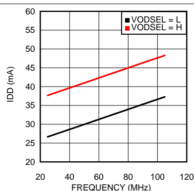
图 18. Typical Current Draw - Single In/Single Out Mode - PRBS-7 Data Pattern
