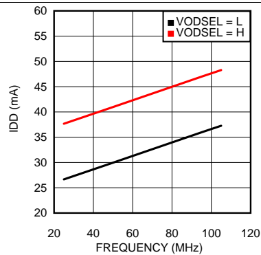
图 13. Typical Current Draw — Single In/Single Out Mode — PRBS-7 Data Pattern
