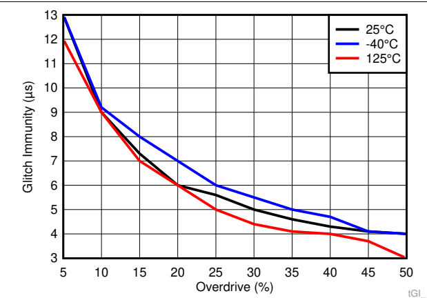
图 27. Glitch Immunity Versus Overdrive for TLV803EA29
