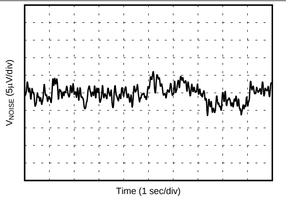
图 43. Internal Reference Noise
