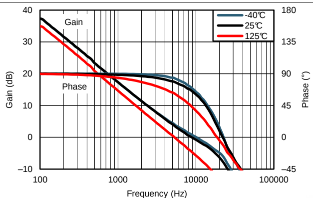
Figure 16. Gain and Phase vs Temperature at 1.8 V
