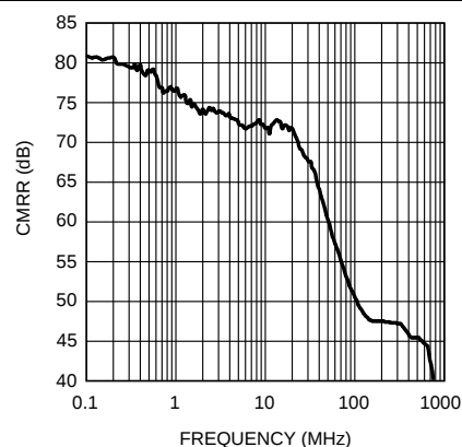
Figure 18. CMRR
