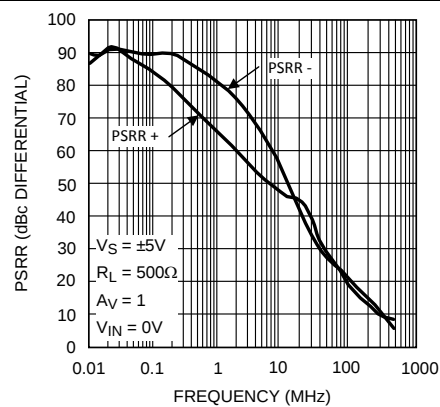
Figure 16. PSRR
