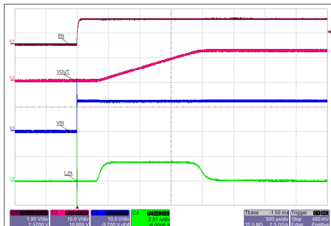
Figure 58. Hot-Plug Start-Up: Output Ramp Without Load on output
