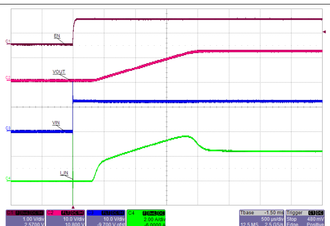
Figure 59. Hot-Plug Start-Up: Output Ramp With Start-up load of 4.8Ω
