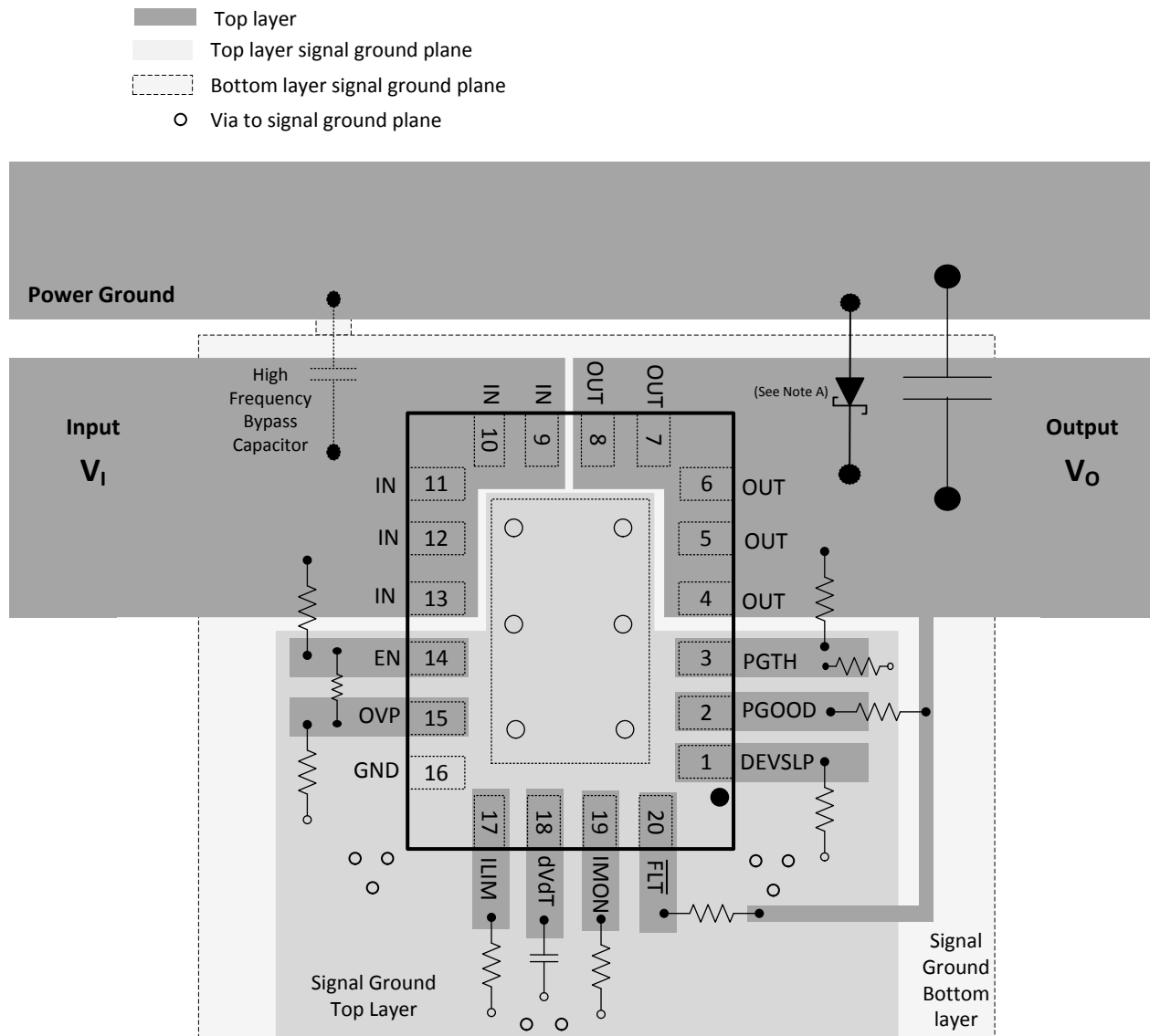
Figure 80. Board Layout
