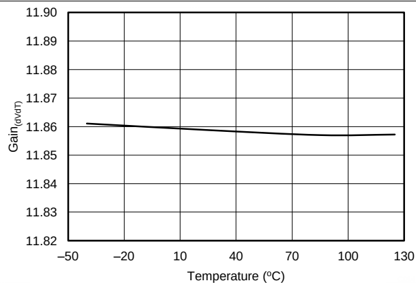
Figure 14. \text{GAIN}_{(dVdT)} vs Temperature
