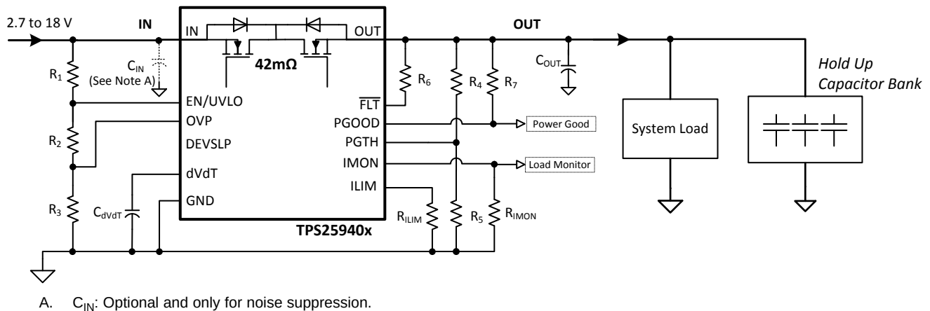
Figure 72. Enterprise SSD – Holdup Capacitor Implementation using TPS25940
