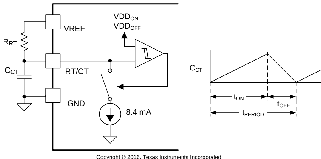
Figure 23. Oscillator Circuit
