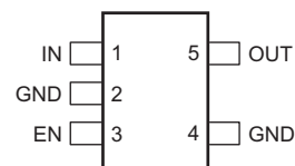
TPS783xxDDC SOT-5 (Top View)
