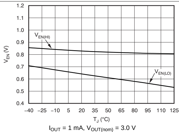
Figure 9. TPS78330 Enable Pin Hysteresis vs Junction Temperature
