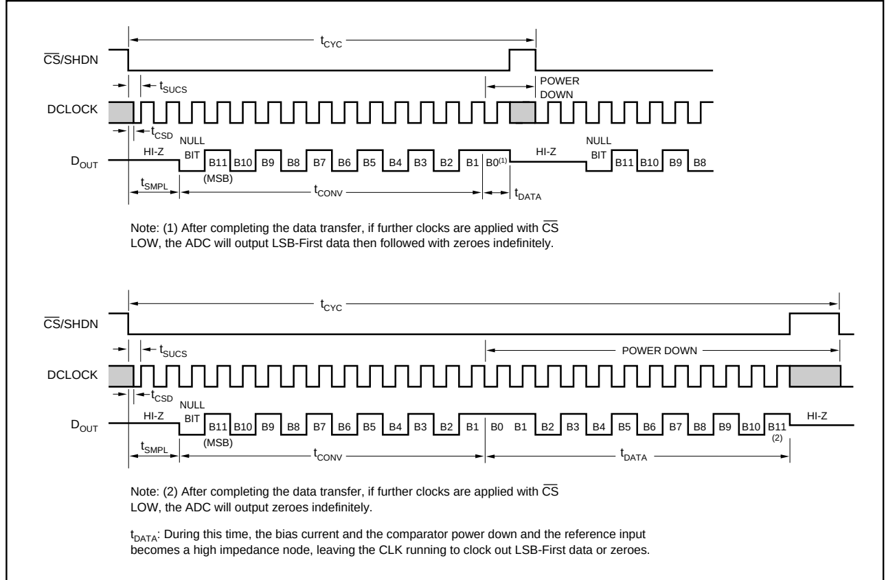
FIGURE 1. ADS7816 Basic Timing Diagrams.
