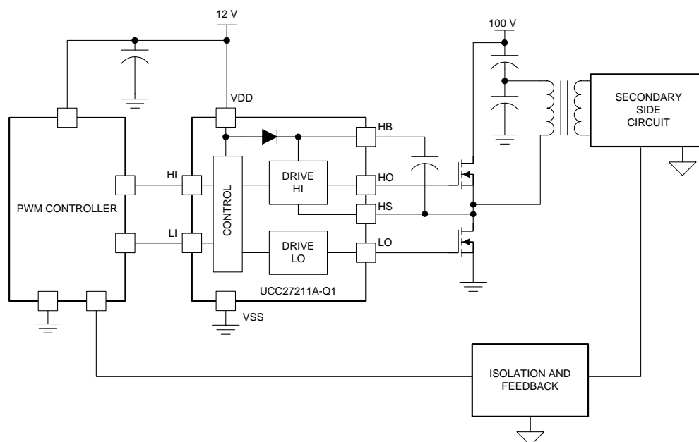
Figure 18. UCC27211A-Q1 Typical Application Diagram
