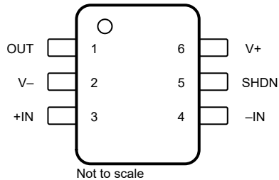
图 5-3. OPA990S DBV and DRL Package (A) 6-Pin SOT-23 and SOT-563 Top View
