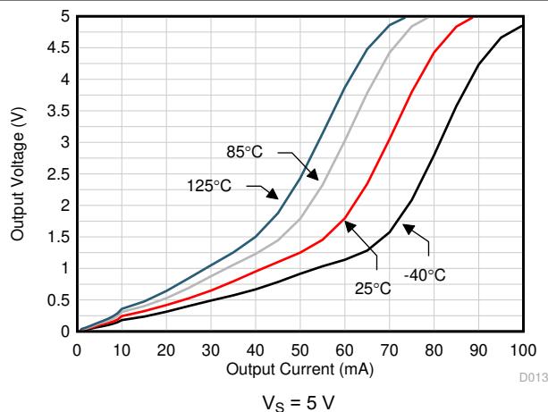
图 6-17. Output Voltage Swing vs Output Current (Sinking)
