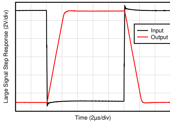
图 6-43. Large-Signal Step Response
