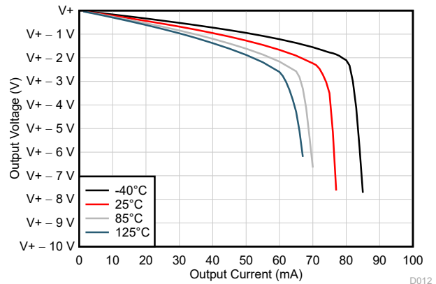
图 6-14. Output Voltage Swing vs Output Current (Sourcing)
