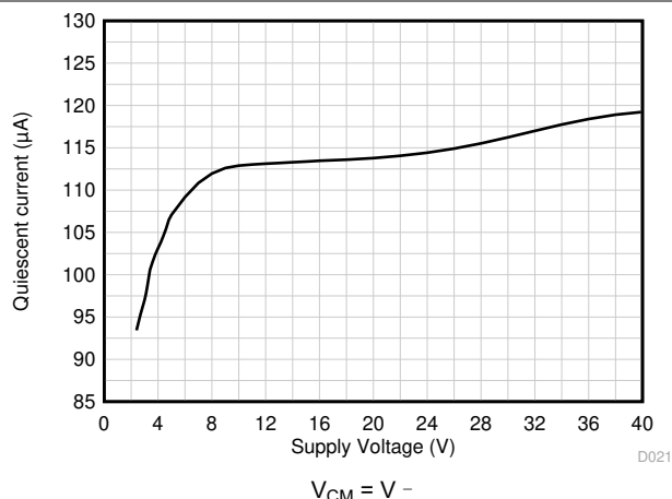
图 6-25. Quiescent Current vs Supply Voltage
