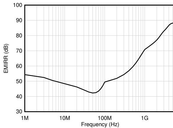
图 6-47. EMIRR (Electromagnetic Interference Rejection Ratio) vs Frequency
