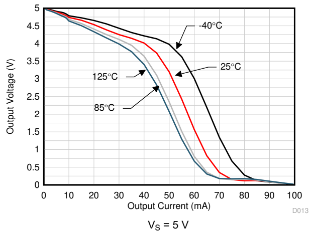
图 6-16. Output Voltage Swing vs Output Current (Sourcing)
