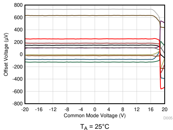
图 6-5. Offset Voltage vs Common-Mode Voltage
