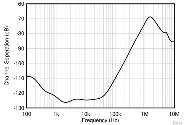
图 6-46. Channel Separation vs Frequency
