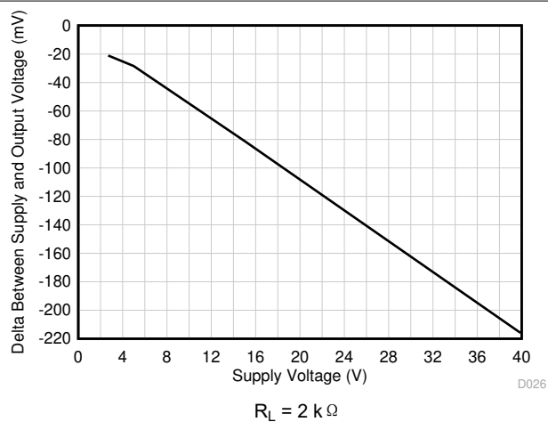
图 6-30. Output Swing vs Supply Voltage, Negative Swing
