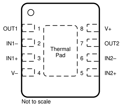
图 5-5. OPA2990 DSG Package (A) 8-Pin WSON With Exposed Thermal Pad Top View
