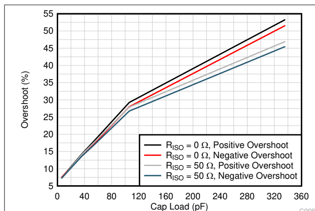
图 7-5. Small-Signal Overshoot vs Capacitive Load (10-mV Output Step, G = 1 )
