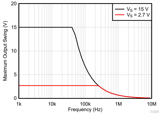
图 6-45. Maximum Output Voltage vs Frequency
