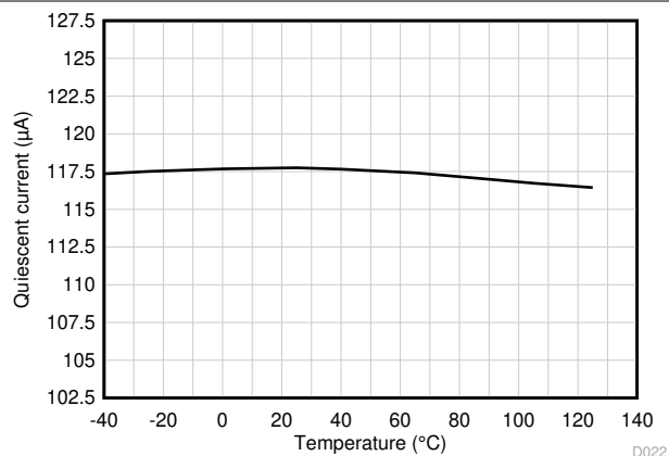
图 6-26. Quiescent Current vs Temperature
