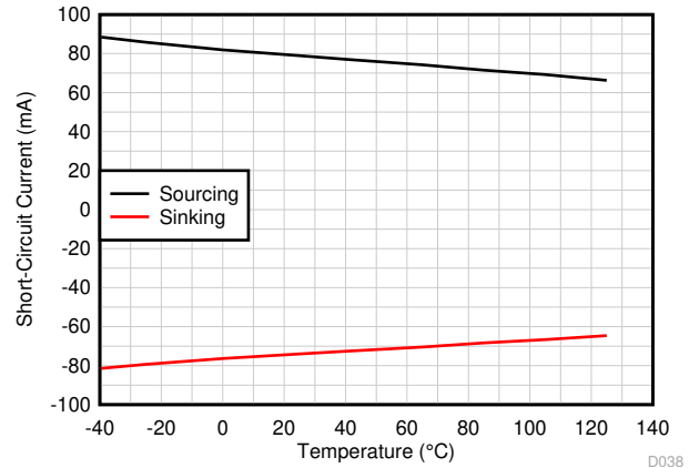
图 6-44. Short-Circuit Current vs Temperature
