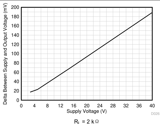
图 6-29. Output Swing vs Supply Voltage, Positive Swing
