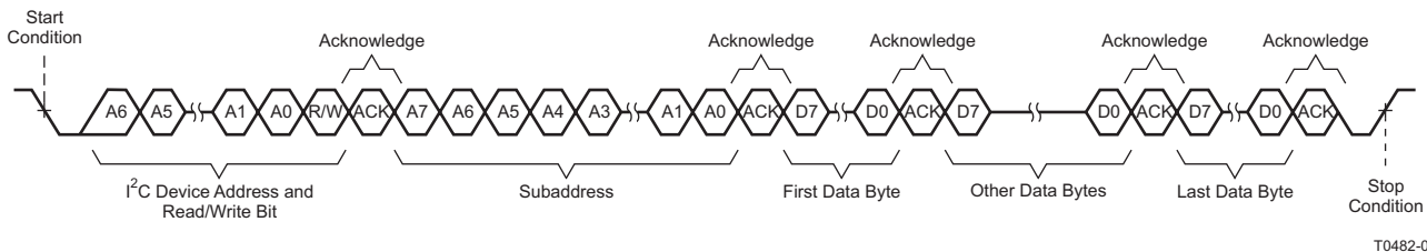
Figure 18. Multiple-Byte Write Transfer
