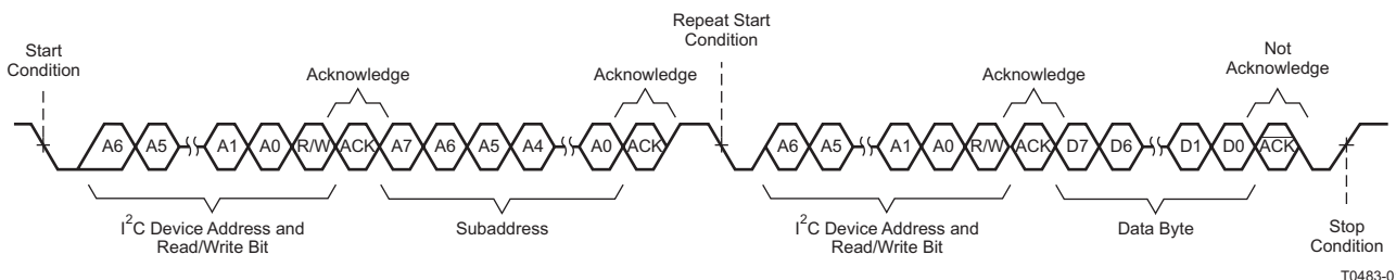
Figure 19. Single-Byte Read Transfer
