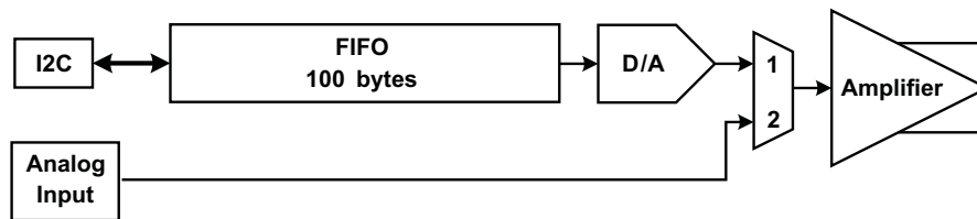
Figure 15. Signal Path
