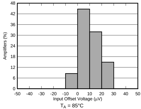
图 3. Offset Voltage Production Distribution
