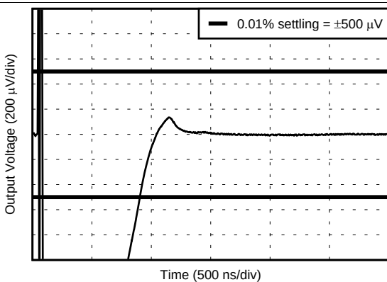
图 43. 0.01% Settling Time
