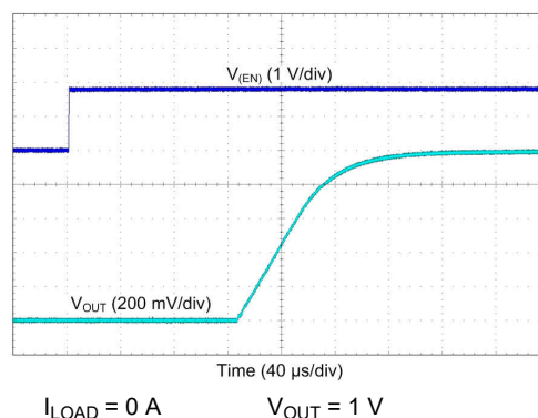
图 8-45. LDO Start-Up
