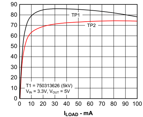
Figure 6-26. Efficiency vs Load Current
