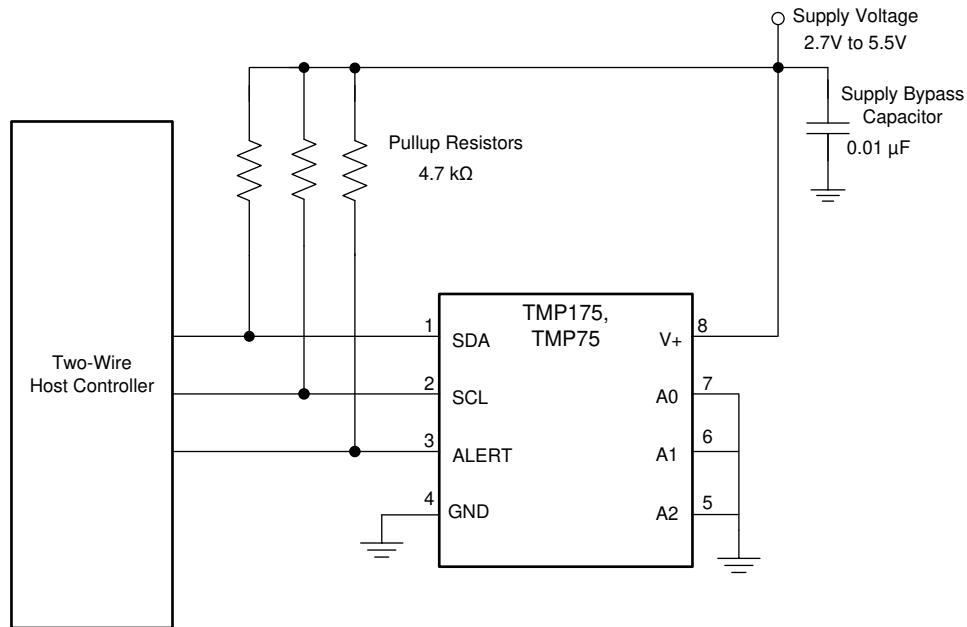
图 8-1. Typical Connections of the TMP175 and TMP75
