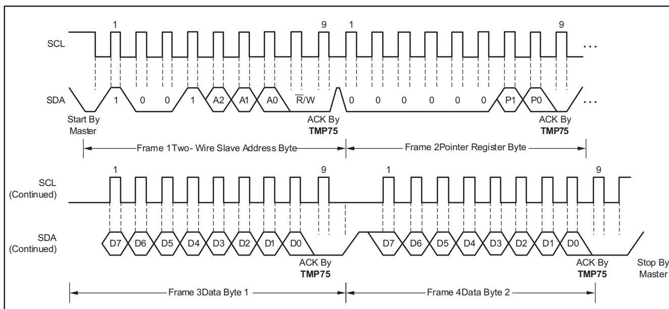
图 7-2. Two-Wire Timing Diagram for the TMP75 Write Word Format
