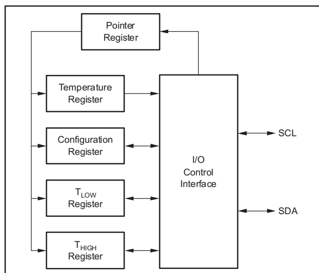
图 7-6. Internal Register Structure of the TMP175 and TMP75
