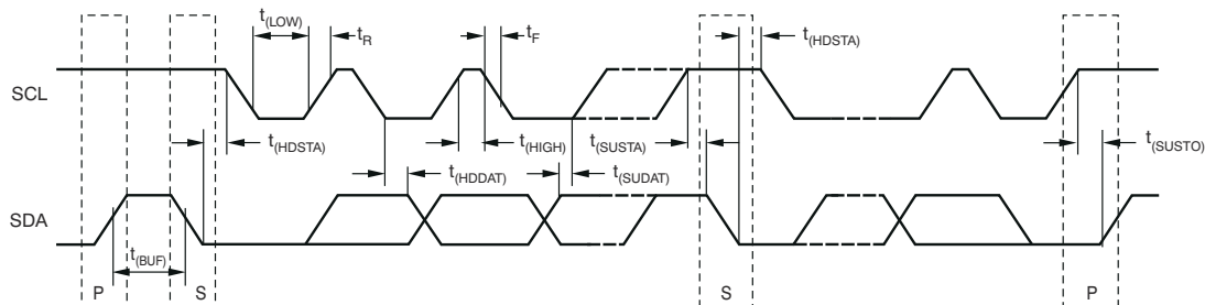
图 7-1. Two-Wire Timing Diagram
