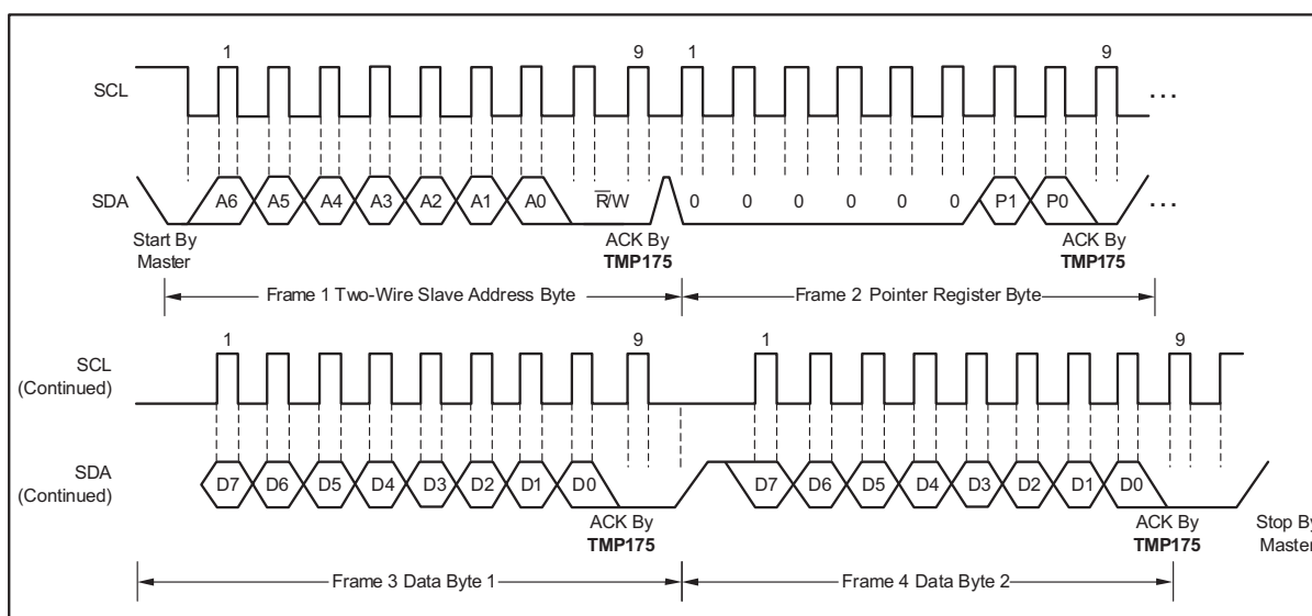
图 7-3. Two-Wire Timing Diagram for the TMP175 Write Word Format
