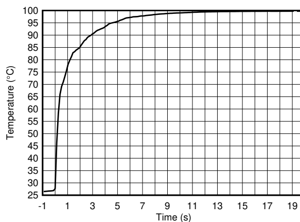
图 8-2. Temperature Step Response
