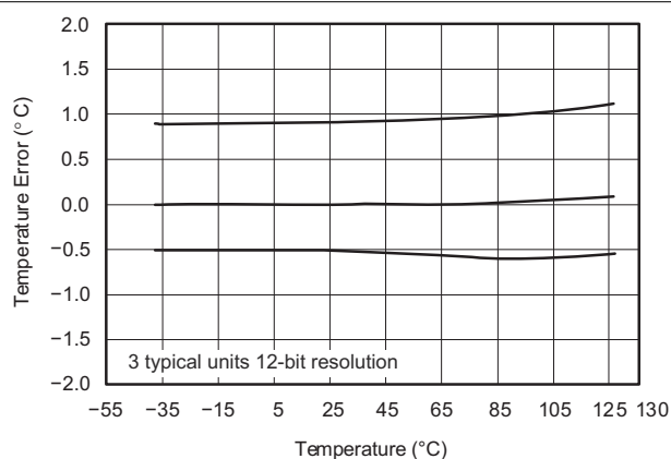
图 6-4. Temperature Accuracy vs Temperature
