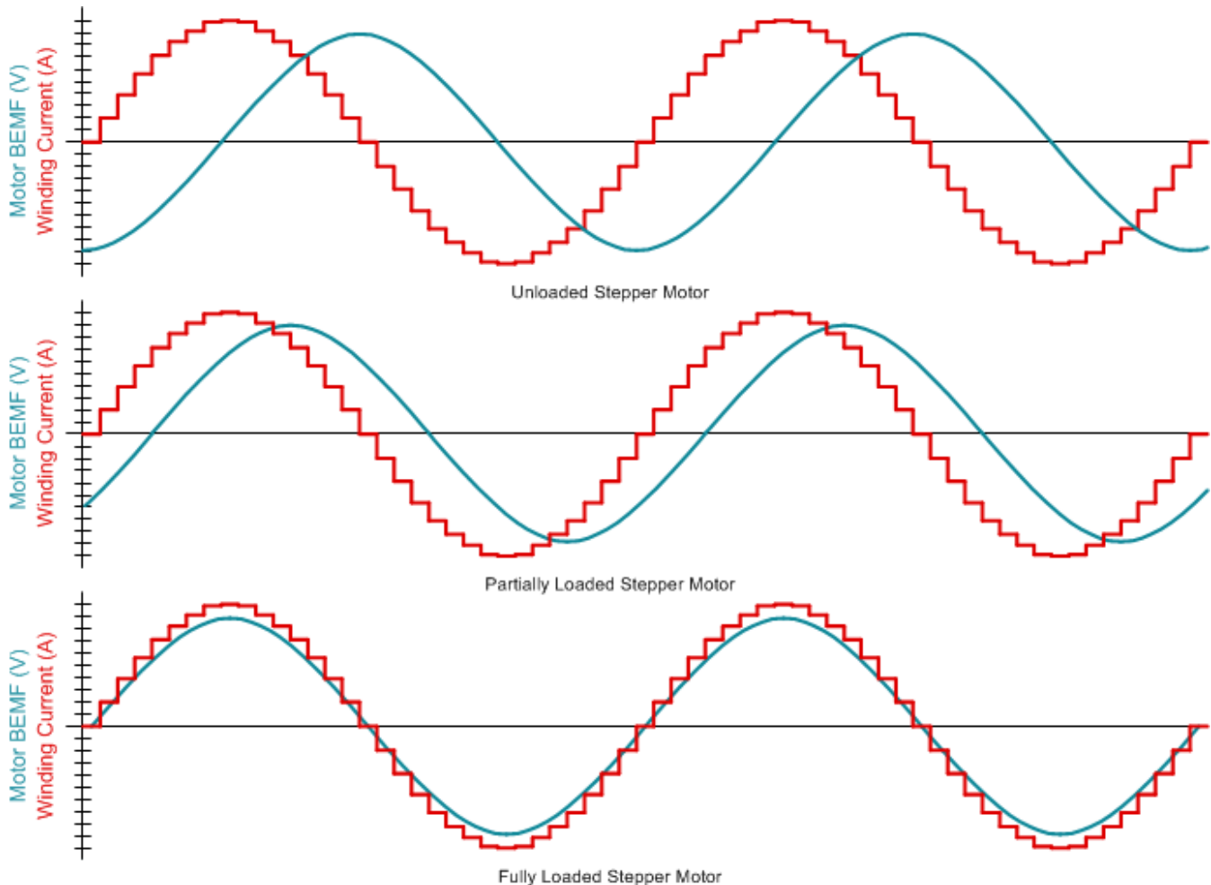
图 31. Stall Detection by Monitoring Motor Back-EMF
