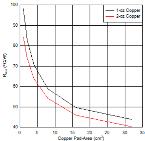
图 70. 4-Layer PCB Junction-to-Ambient Thermal Resistance (R θJA ) vs Copper Area
