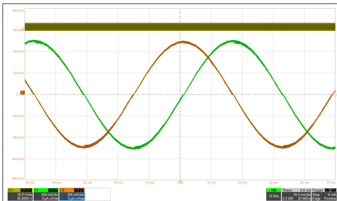
图 58. 1/32 Microstepping With smart tune Ripple Control Decay
