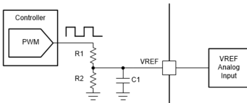
图 14. Controlling VREF With a PWM Resource
