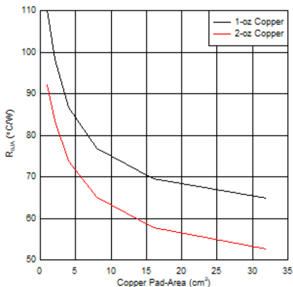
图 68. 2-Layer PCB Junction-to-Ambient Thermal Resistance (R θJA ) vs Copper Area
