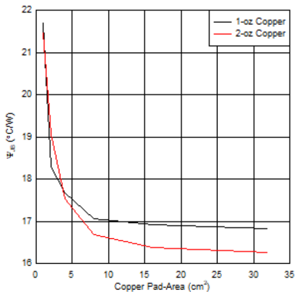
图 71. 4-Layer PCB Junction-to-Board Characterization Parameter (Psi JB ) vs Copper Area
