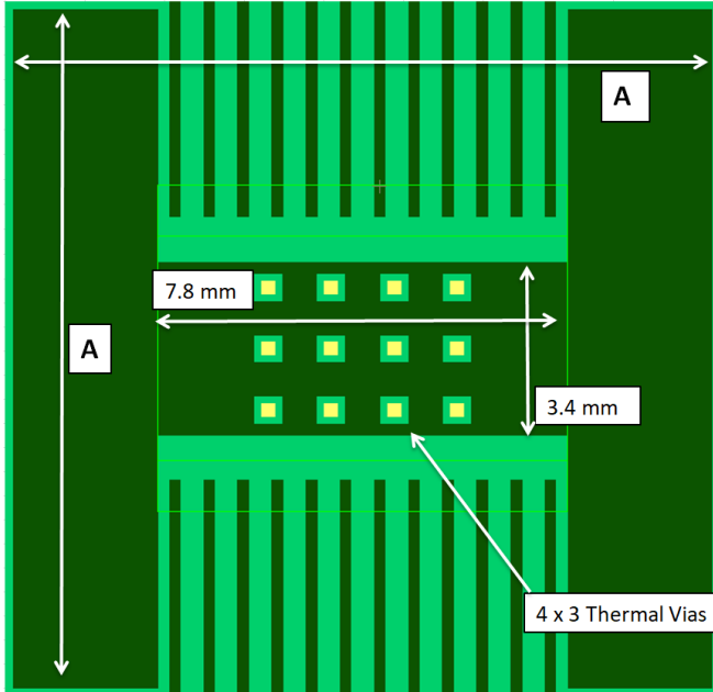
图 62. PCB - Top Layer (4/2-Layer PCB) for HTSSOP Package
