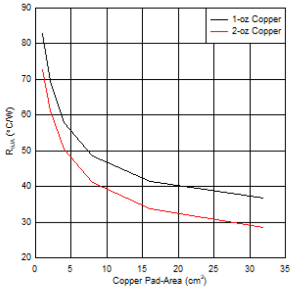
图 64. 2-Layer PCB Junction-to-Ambient Thermal Resistance ( R_{\theta JA} ) vs Copper Area
