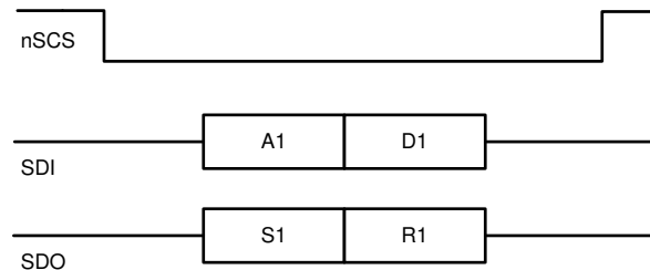
图 33. SPI Transaction Between MCU and the device
