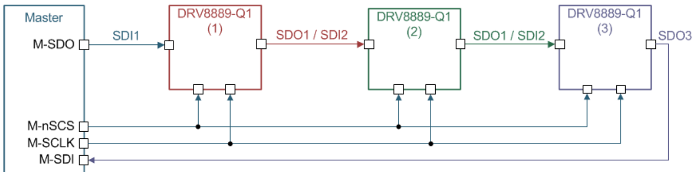
图 35. Three DRV8889-Q1 Devices Connected in Daisy Chain
