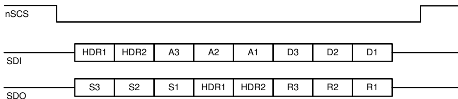
图 37. SPI Data Sequence for Three Devices
