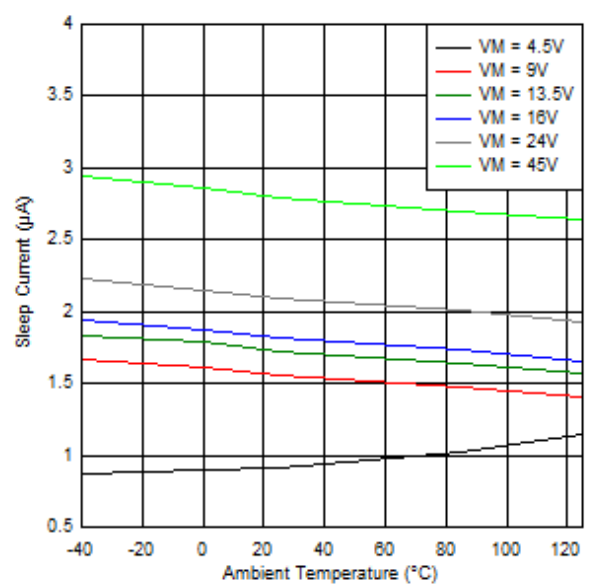
图 4. Sleep Current over Temperature
