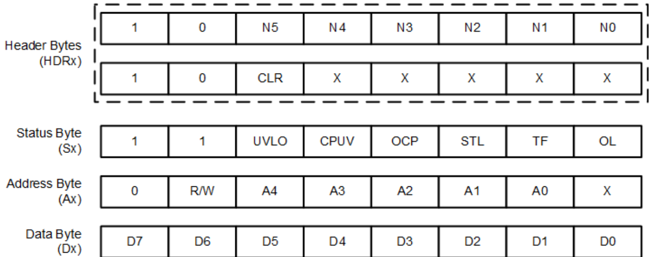
图 39. Contents of Header, Status, Address, and Data Bytes for DRV8889-Q1
