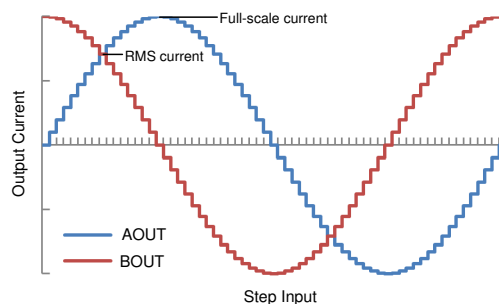
图 11. Full-Scale and RMS Current
