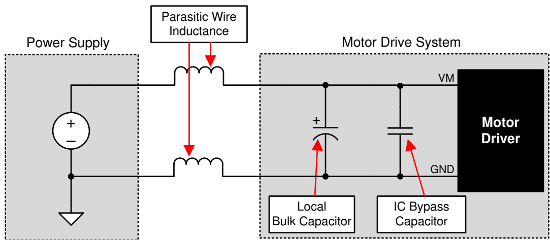
图 72. Example Setup of Motor Drive System With External Power Supply
