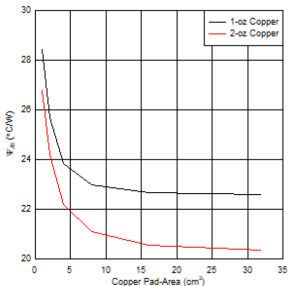
图 69. 2-Layer PCB Junction-to-Board Characterization Parameter (Psi JB ) vs Copper Area
