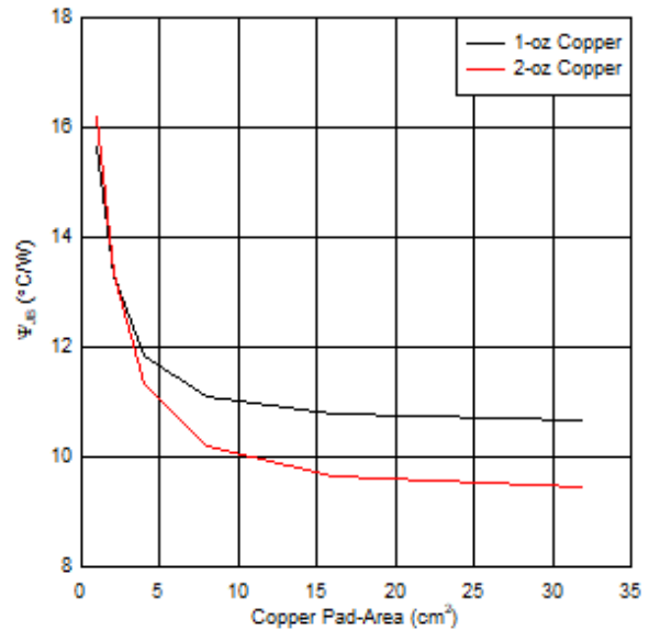
图 65. 2-Layer PCB Junction-to-Board Characterization Parameter ( \Psi_{JB} ) vs Copper Area
