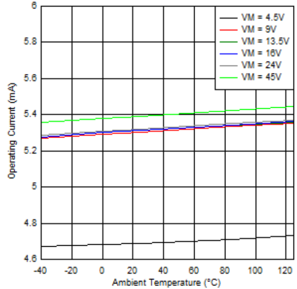
图 6. Operating Current over Temperature
