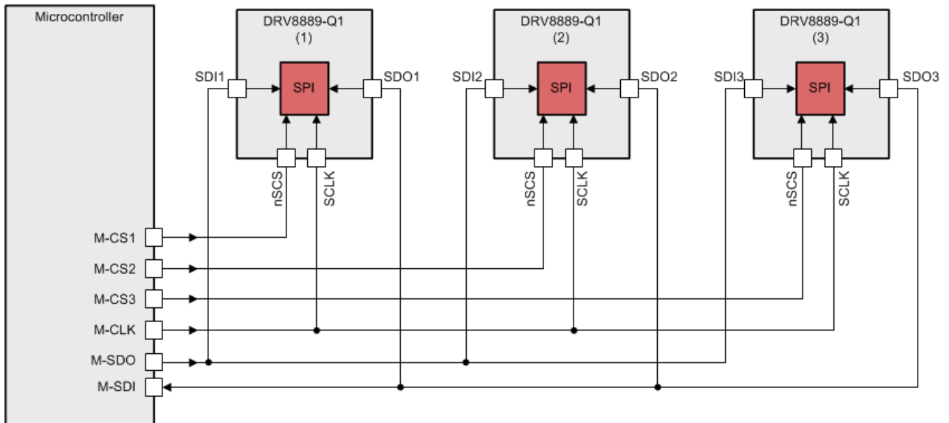
图 34. Three DRV8889-Q1 Devices Connected in Parallel Configuration
