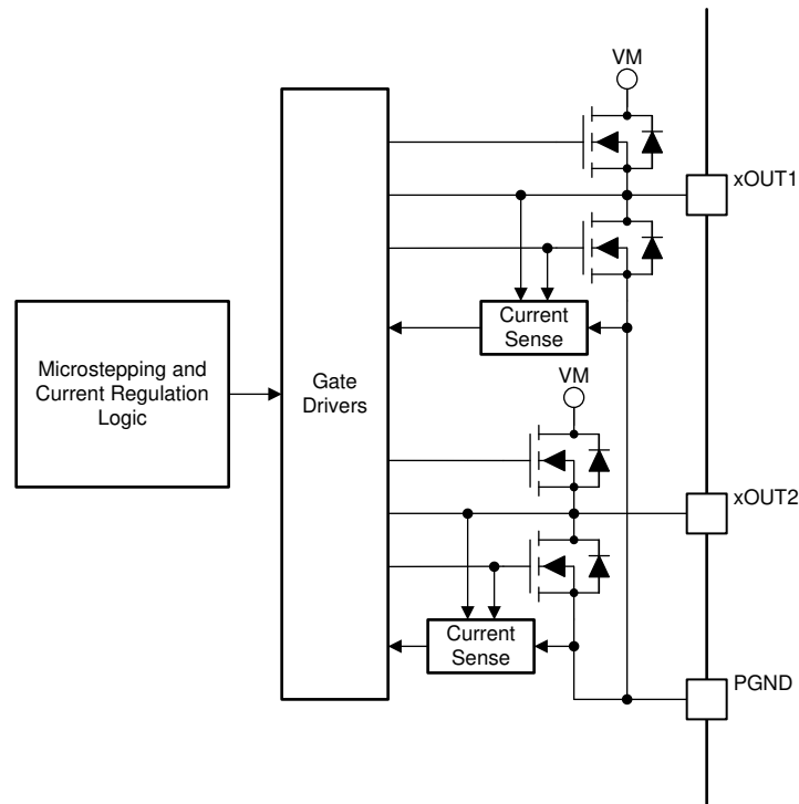
图 12. PWM Motor Driver Block Diagram
