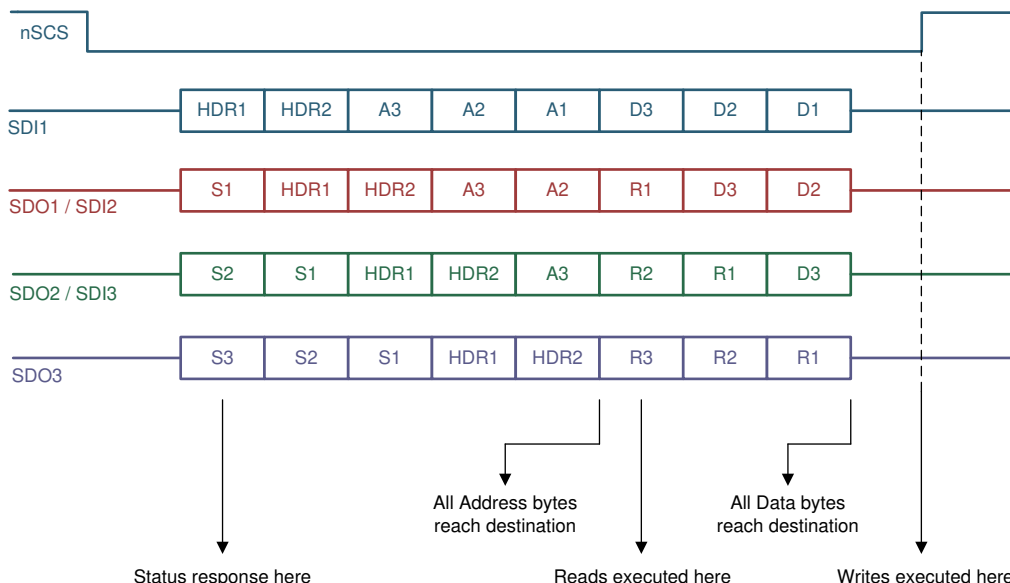
图 36. SPI Frame With Three Devices
