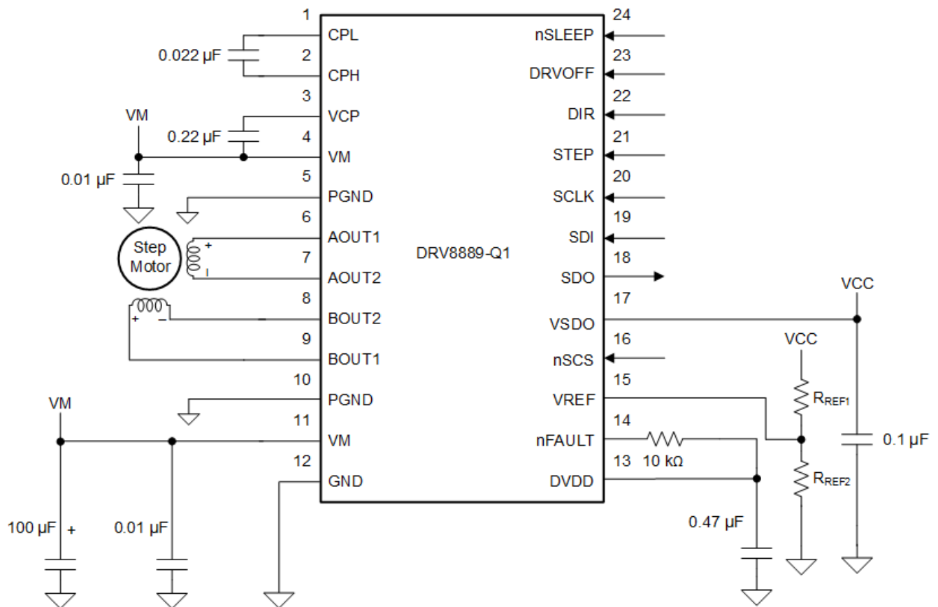
图 52. Typical Application Schematic (HTSSOP package)
