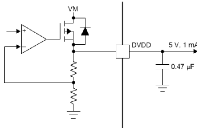
图 25. Linear Voltage Regulator Block Diagram
