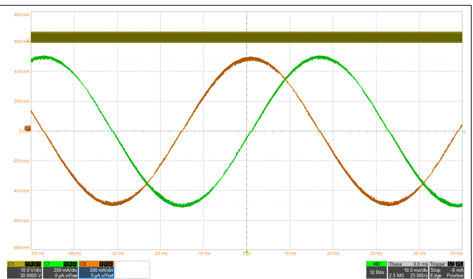
图 61. 1/256 Microstepping With smart tune Dynamic Decay
