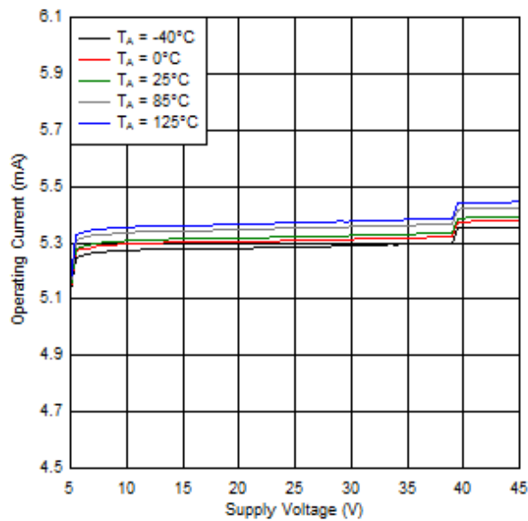
图 5. Operating Current over VM
