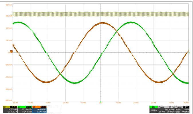
图 59. 1/32 Microstepping With smart tune Dynamic Decay
