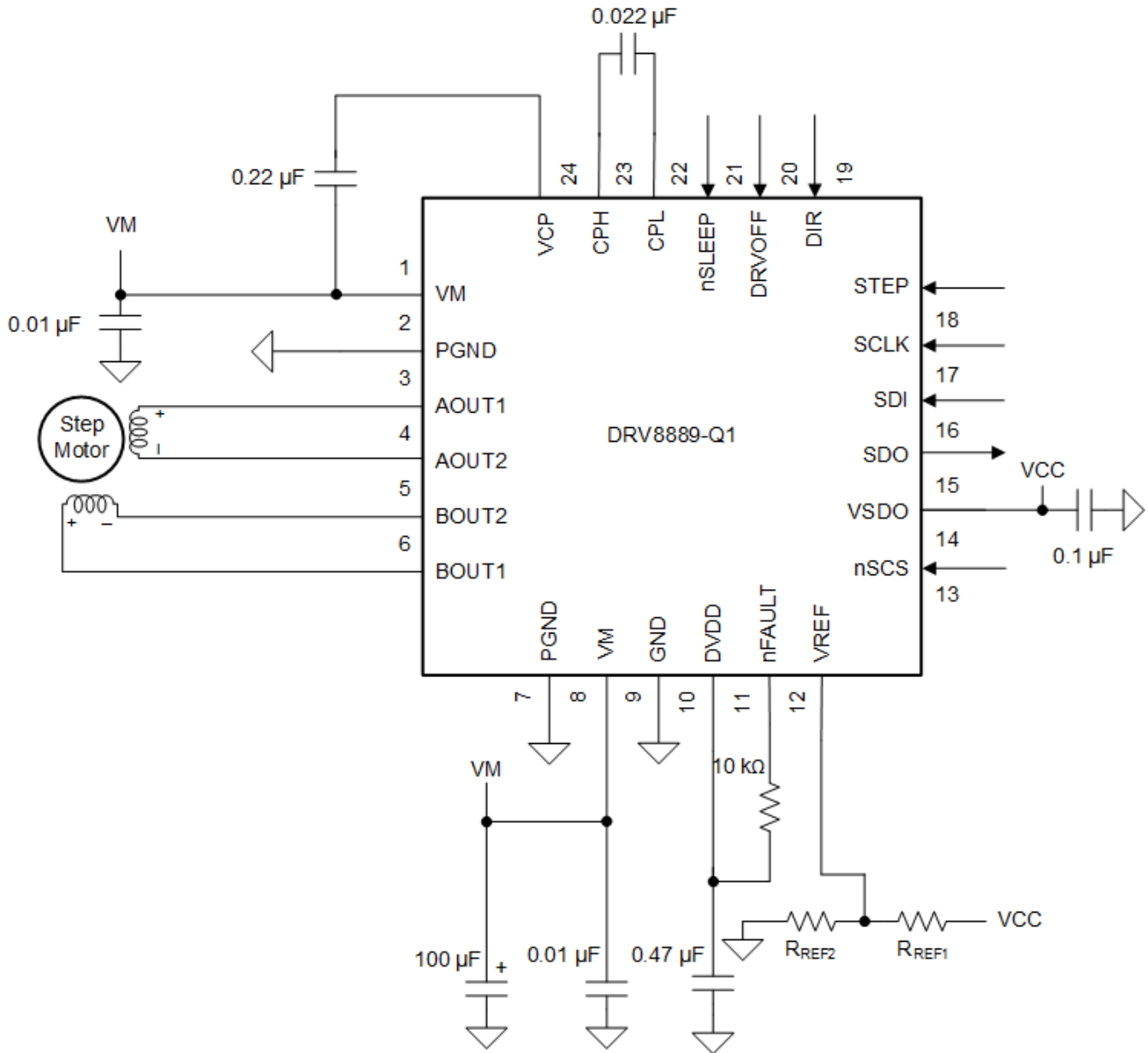
图 53. Typical Application Schematic (VQFN package)
