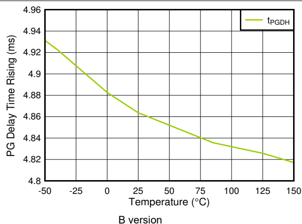
图 6-25. t_{PGDH} vs Temperature (For TPS746B Only)
