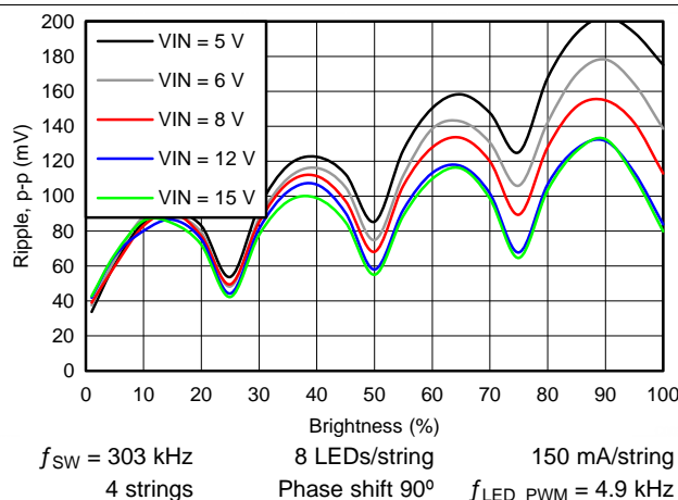
Figure 7. Boost Ripple
