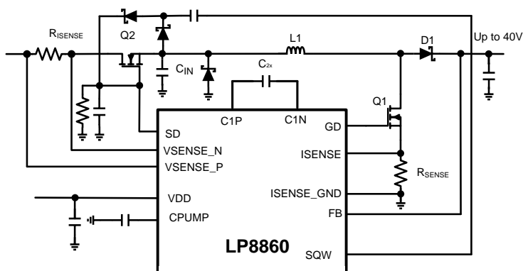
Figure 24. V_{\text{RAIL}} Multiplied by 4
