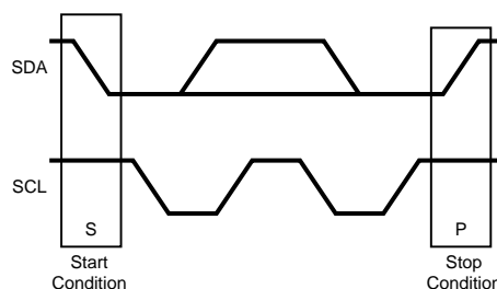
Figure 49. Stop and Start Conditions
