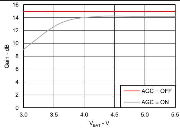
图 21. Gain vs Supply Voltage
