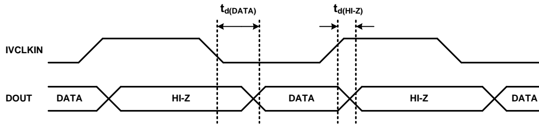
图 49. DOUT Timing in PDM Mode (Data on IVCLKIN Low)
