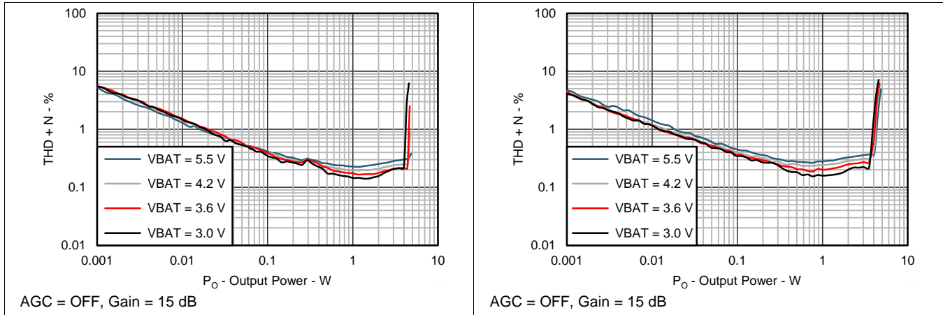
图 15. I-Sense THD+N vs Output Power (8Ω)
