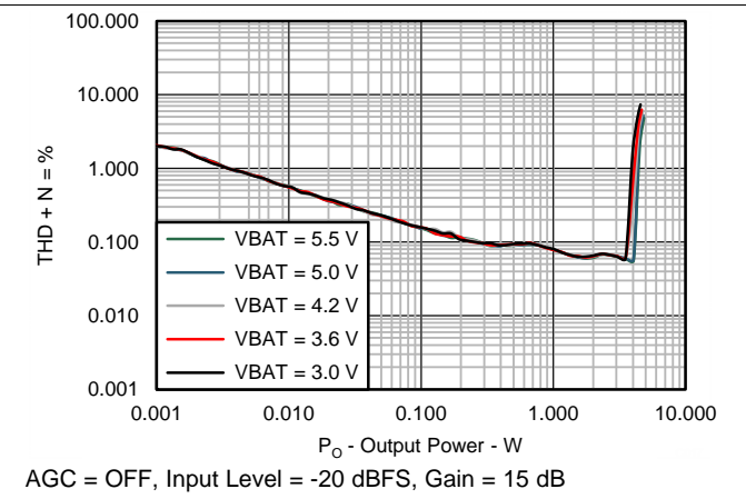
图 16. I-Sense THD+N vs Output Power (6Ω)
