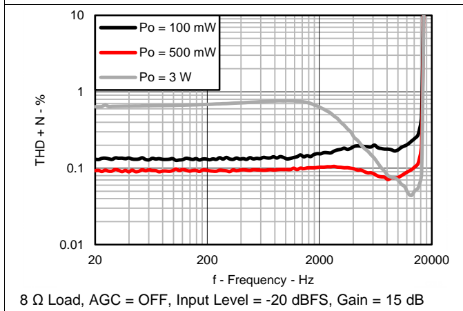
图 17. I-Sense THD+N vs Frequency (8Ω)
