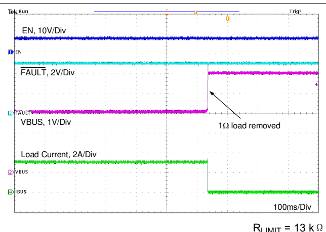
图 11-25. 1-Ω Load Recovery Without External FET
