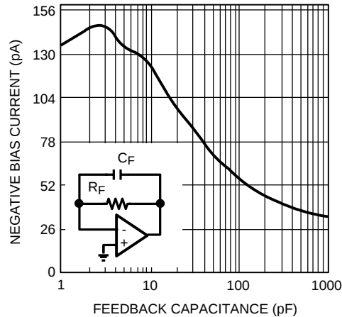
Figure 42. Input Bias Current vs. C_F with R_F = 1 G \Omega
