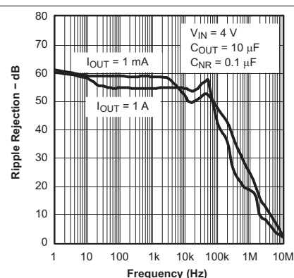
Figure 27. TPS79630 Ripple Rejection vs Frequency
