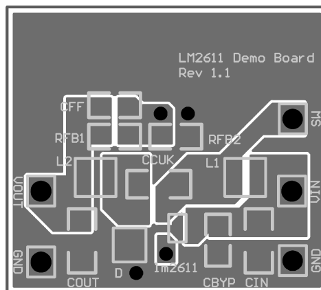
Figure 36. Example Layout Top
