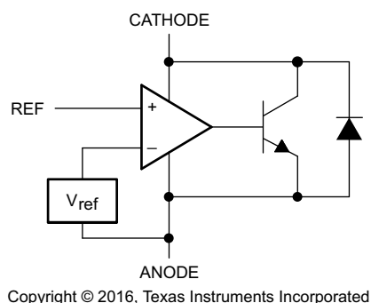
Figure 23. Equivalent Schematic
