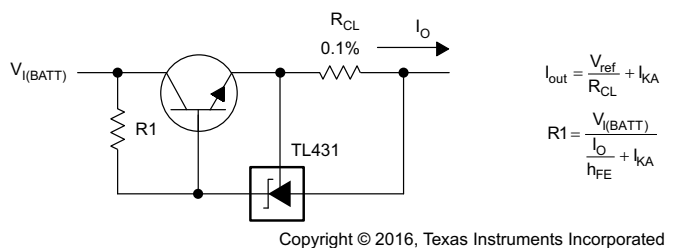
Figure 37. Voltage Monitor
