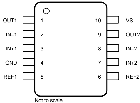
INA2181: DGS Package 10-Pin VSSOP Top View
