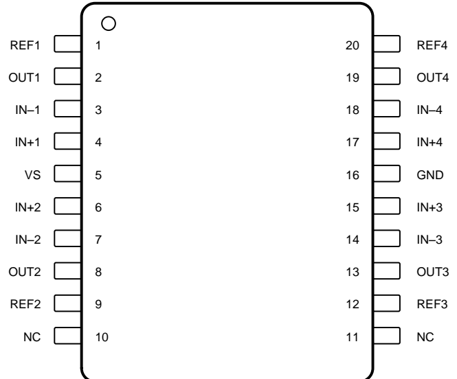
INA4181: PW Package 20-Pin TSSOP Top View
