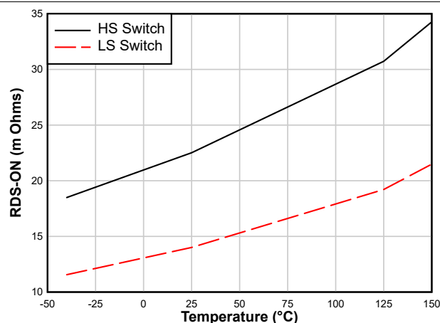
图 7-3. High-side and Low-side Switches R_{DS\_ON}
