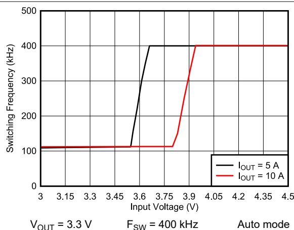
图 9-26. Frequency Dropout
