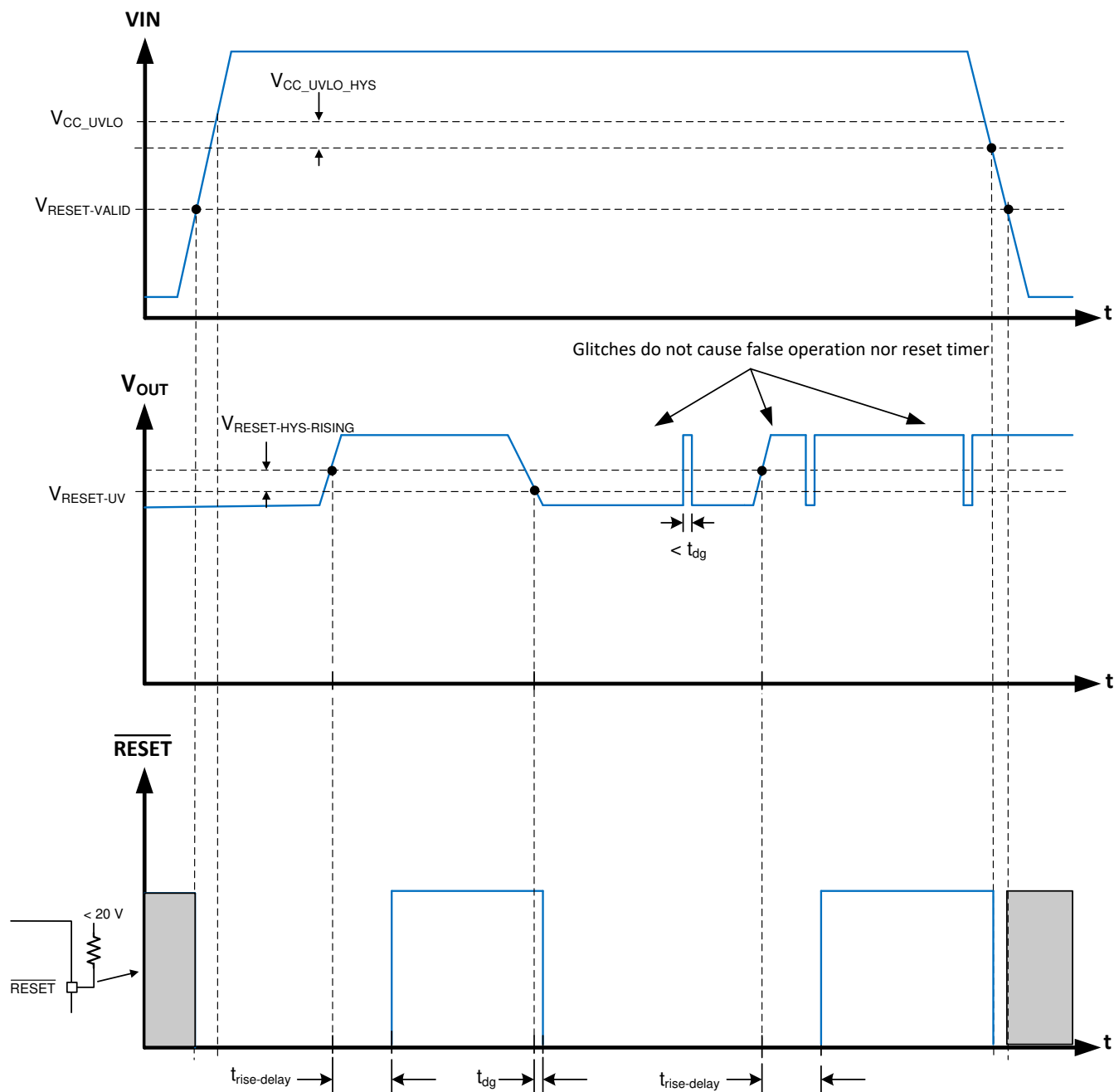
图 8-8. \overline{RESET} Timing Diagram (Excludes OV Events)
