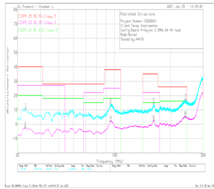
图 9-53. Radiated EMI Bicon Horizontal versus CISPR25 Class 5 Limits
