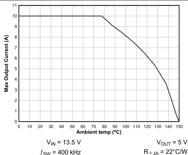
图 9-3. Maximum Output Current versus Ambient Temperature
