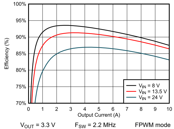
图 9-12. Efficiency
