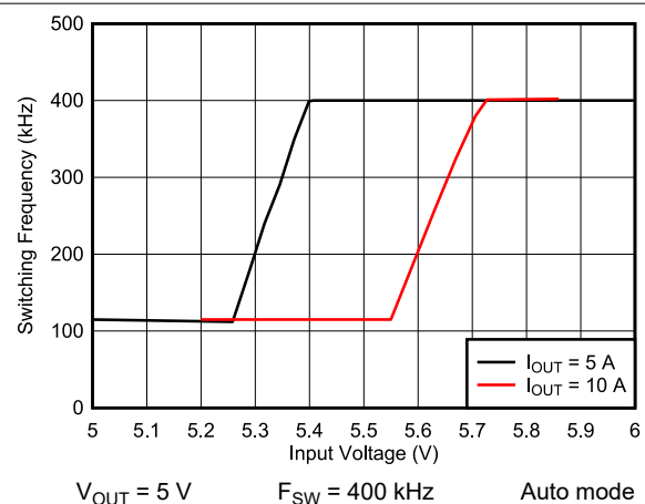
图 9-25. Frequency Dropout
