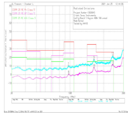
图 9-48. Radiated EMI Bicon Vertical versus CISPR25 Class 5 Limits
