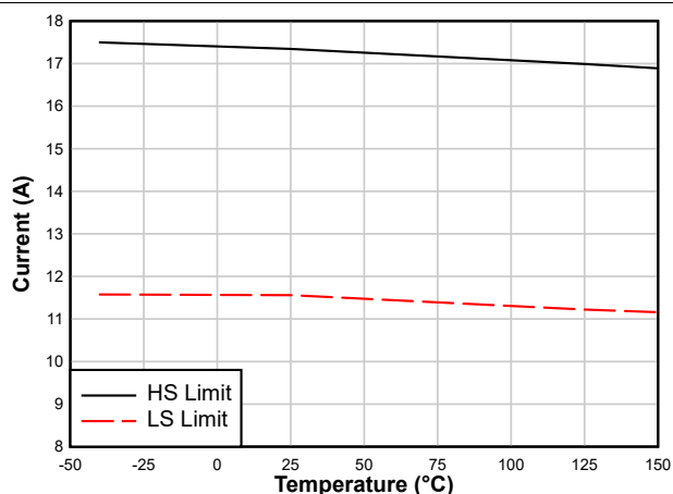
图 7-4. High-side and Low-side Current Limits
