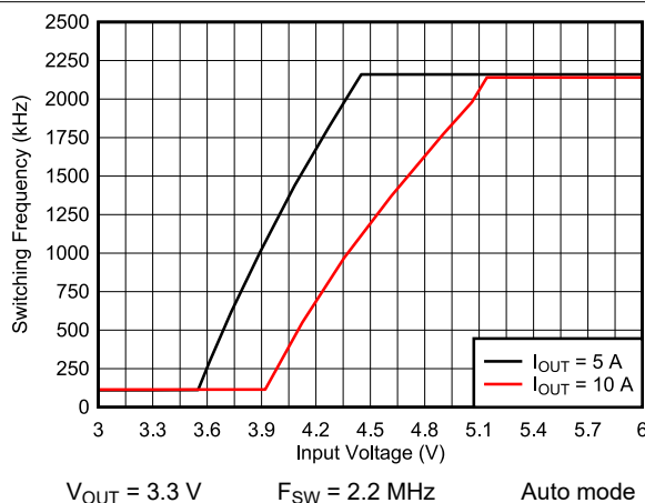
图 9-28. Frequency Dropout
