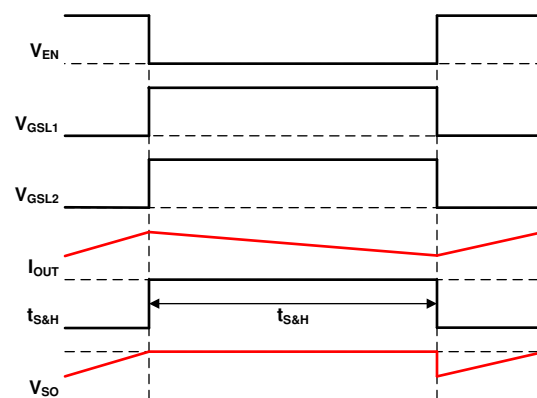
Figure 7-12. DRV8705-Q1 Amplifier Sample & Hold Example
