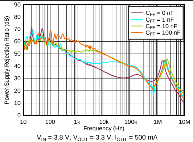
图 38. PSRR vs Frequency and C_{FF}
