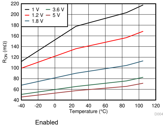
图 6-1. ON-Resistance vs Temperature
