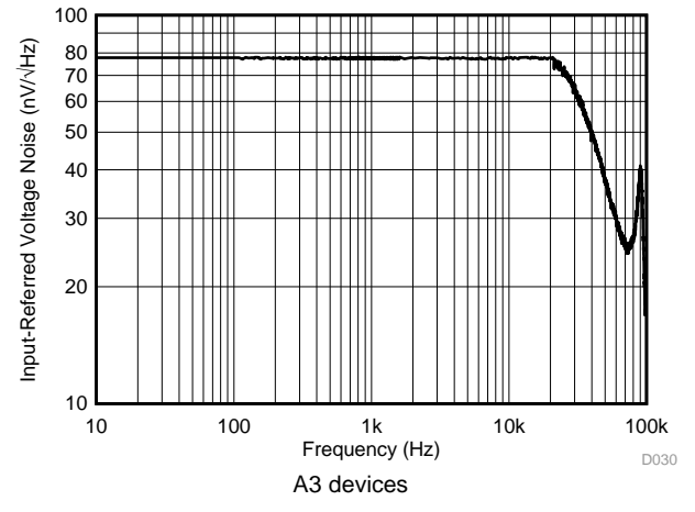
图 18. Input-Referred Voltage Noise vs Frequency
