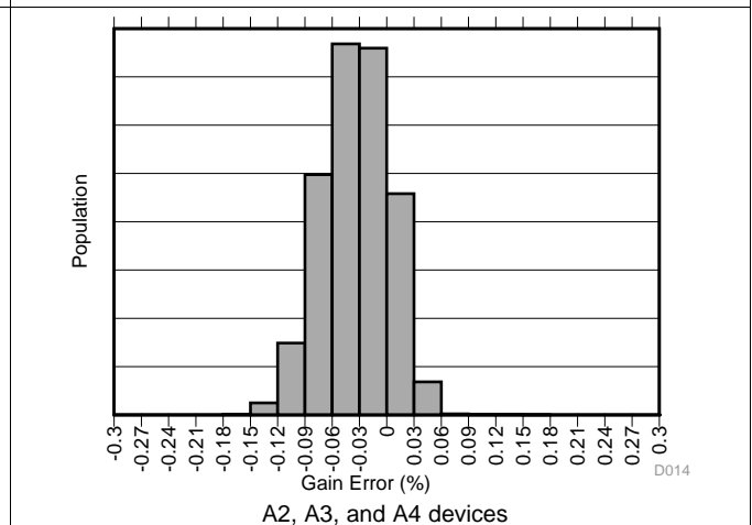
图 6. Gain Error Production Distribution
