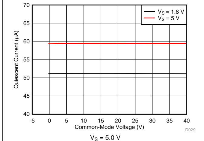
图 17. Quiescent Current vs Common Mode Voltage
