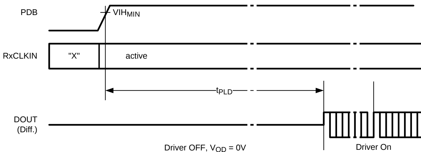
Figure 9. DS92LV0411 Lock Time
