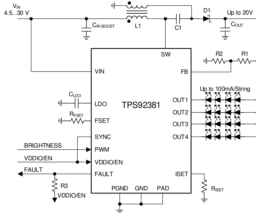
图 9-4. SEPIC Mode, 4 Strings 100 mA per String Configuration
