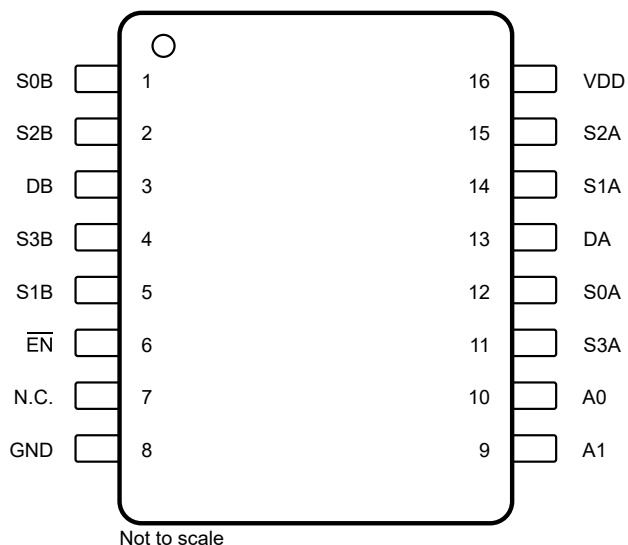
Figure 6-4. TMUX1309: PW Package 16-Pin TSSOP Top View
