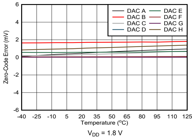
Figure 7-20. Zero-Code Error vs Temperature
