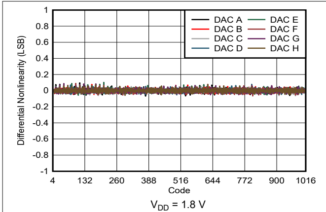
Figure 7-8. Differential Nonlinearity vs Digital Input Code
