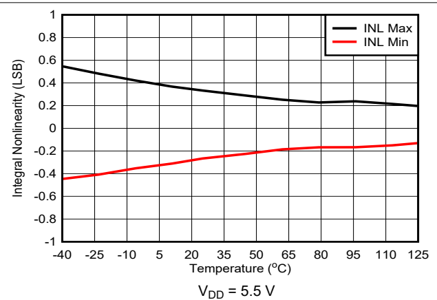
Figure 7-5. Integral Nonlinearity vs Temperature
