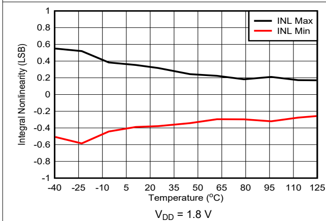
Figure 7-4. Integral Nonlinearity vs Temperature
