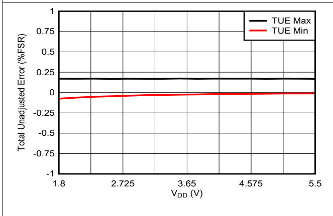
Figure 7-18. Total Unadjusted Error vs Supply Voltage
