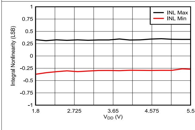
Figure 7-6. Integral Nonlinearity vs Supply Voltage
