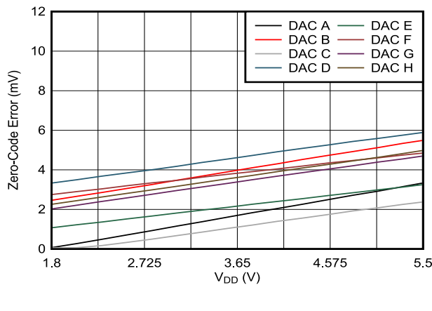
Figure 7-22. Zero-Code Error vs Supply Voltage
