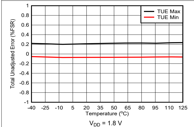
Figure 7-16. Total Unadjusted Error vs Temperature
