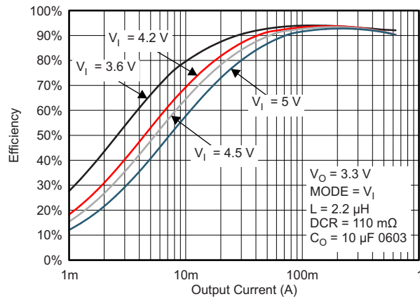
Figure 9. Efficiency (PWM Mode) vs Output Current
