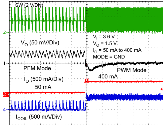
Figure 31. Load Transient (PFM Mode to PWM Mode)
