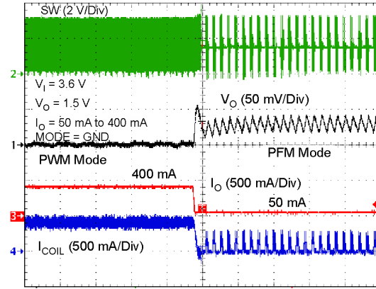
Figure 32. Load Transient (PWM Mode to PFM Mode)
