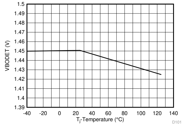
图 2. VINAC Brownout Detection Threshold
