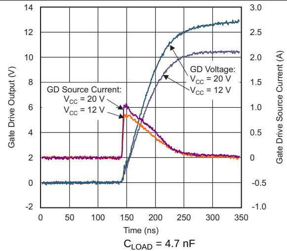
图 12. Gate Drive Rising vs Time
