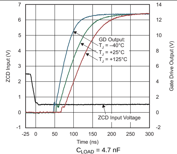
图 14. Gate Drive Rising and Delay From ZCD Input vs Time
