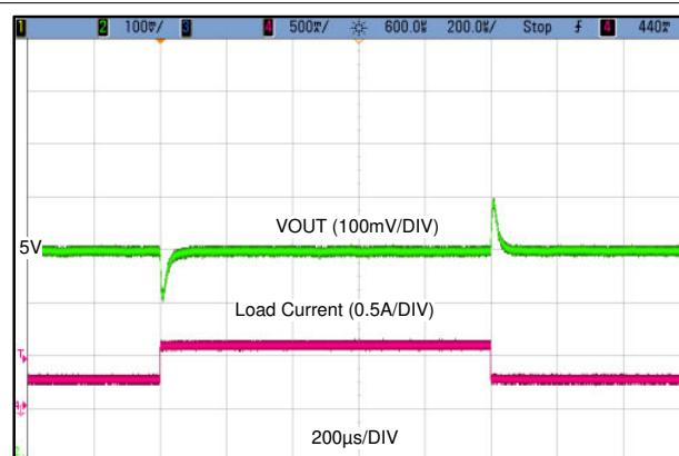
LMR36506R V_{OUT} = 5V Fixed 400 kHz
