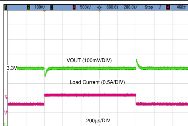
LMR36506R3 V_{OUT} = 3.3V Fixed 1 MHz
