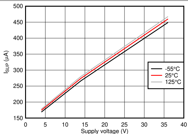
图 7-4. Recessive I_{SUP} vs V_{SUP} and Temperature
