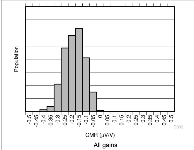
图 7-3. Common-Mode Rejection Ratio Production Distribution
