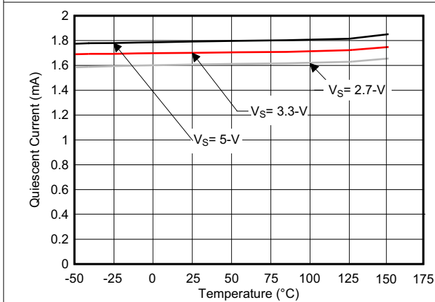
图 7-17. Quiescent Current vs Temperature
