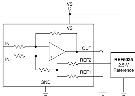
图 8-7. Mid-External Reference Output
