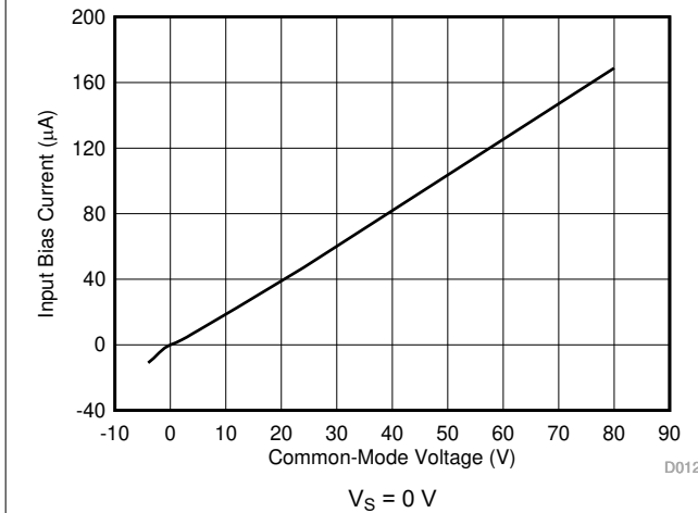
图 7-15. Input Bias Current vs Common-Mode Voltage
