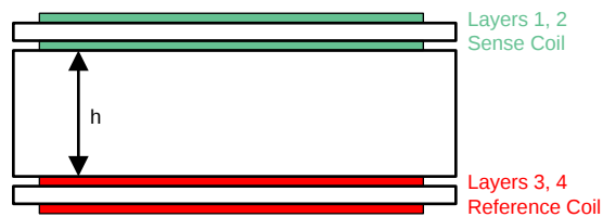
图 21. Stacked Coil Separation (PCB Side View)
