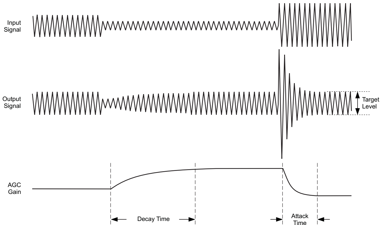
图 18. Typical Operation of the AGC Algorithm During Speech Recording
