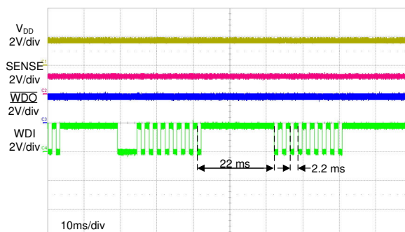
图 8-10. Window Watchdog Timing
