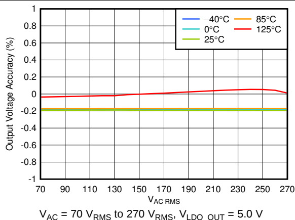
图 1. V_{LDO\_OUT} Accuracy vs V_{AC} Supply
